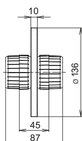
Coupling element, including screw set BN 528101
