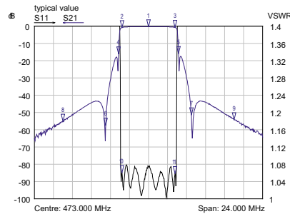
Typical diagram AS8074
