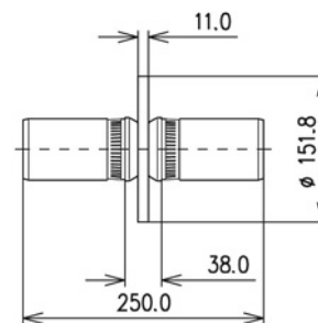
Inner support BN 532784
