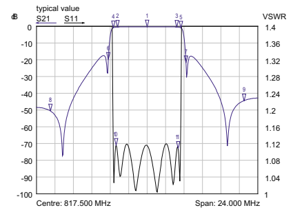
Typical diagram AS6290
