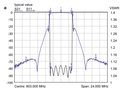
Typical diagram AS8094
