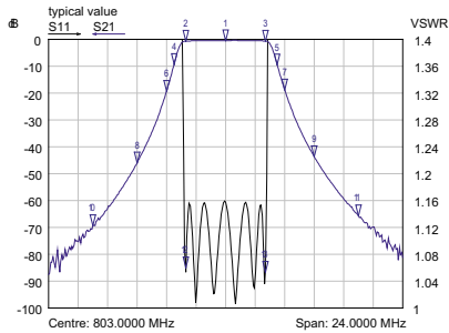
Typical diagram AS6082
